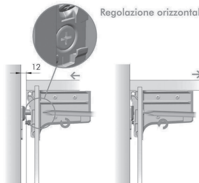
Horizontal adjustment 12 mm
