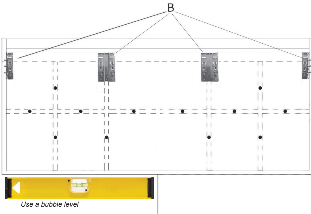
Image 2 HANGERS “B” TO BE HOOKED TO THE BRACKETS “A”
